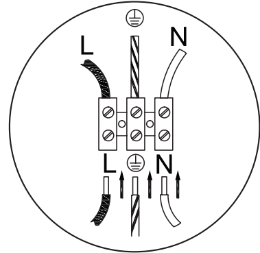
3. Details of terminal wiring.
